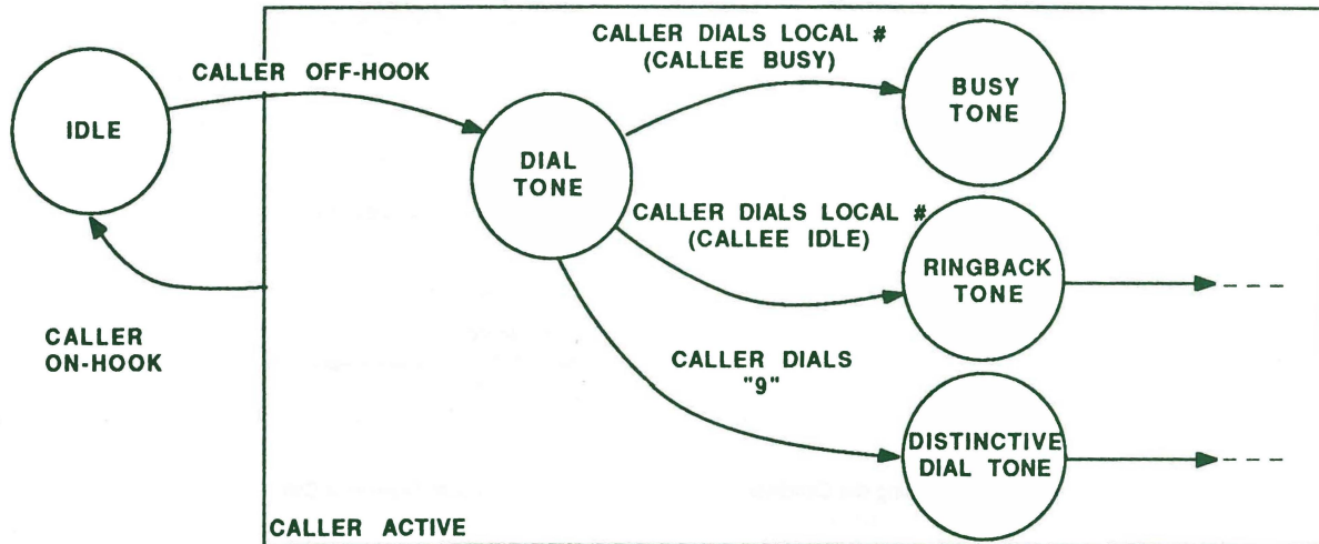
FIGURE 12. Using the Superstate Extension in Telephony
